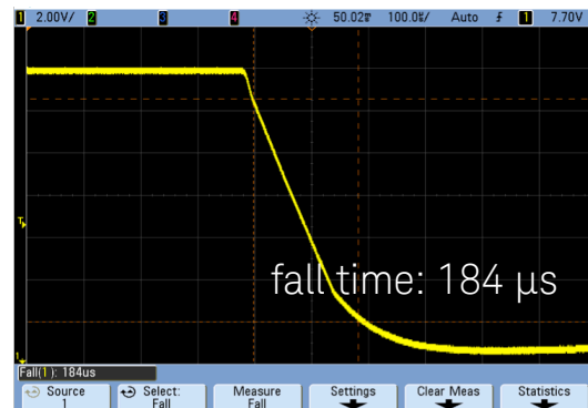
Figure 5. Interrupt pulse fall time measurement of < 200 μs
