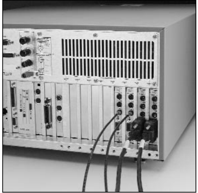
Remote PreAmp Cables (4200-RPC) provide analog signal paths and digital control when the 4200-PA is placed in a remote location.
