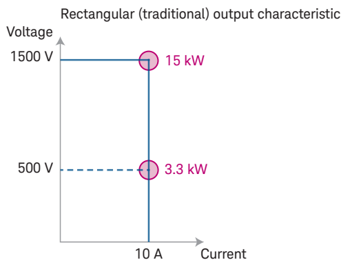
Figure 5. Rectangular output characteristic
