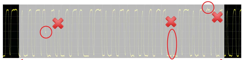
Figure 4: Other vendor's oscilloscope with 50,000 waveforms/second. A long dead time decreases your chances of capturing infrequent events.
