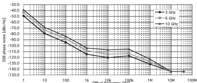
Figure 2-3. E5052A downconverter LO phase noise (typical)
