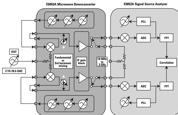
Figure 2-1. E5053A with E5052A block diagram
