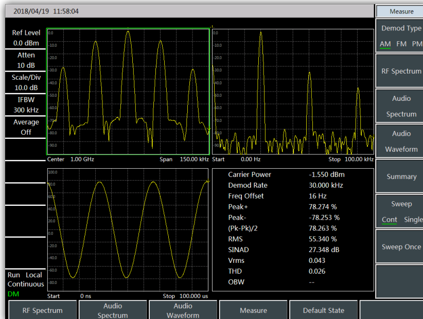
➤ AM/FM/PM Analyzer
