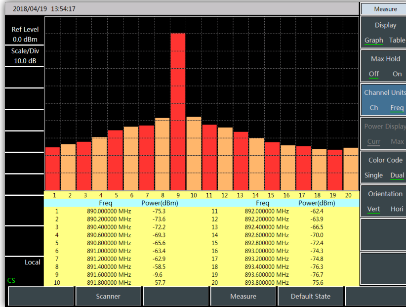
➤ Channel Scanner
