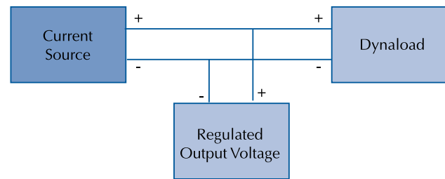
SHUNT VOLTAGE REGULATION
