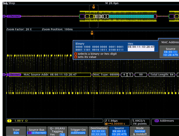
DPO4ENET triggering on a specific 10BASE-T MAC source address.
