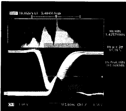
The horizontal histogram of the selected region of the waveform shows the character of a metastable flip-flop output.
