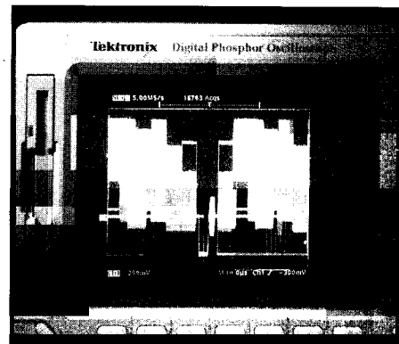
The same composite video signal, captured with a Digital Phosphor Oscilloscope, shows all the details of this complex waveform, in real-time.
