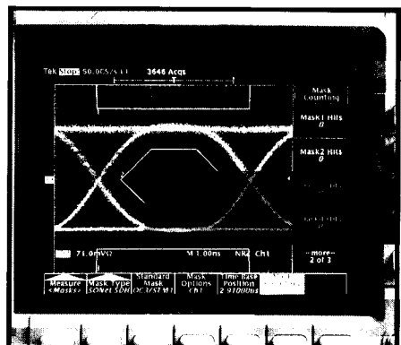
A SONET/SDH (OC-3/STM-1) signal is compared with the standard mask, showing a compliant waveform.
