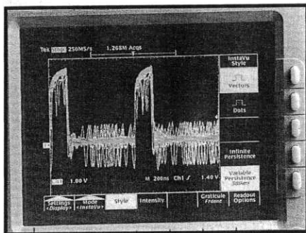
The same waveform, captured with InstaVu acquisition, uncovers detail in the signal which goes unnoticed by a common DSO.
