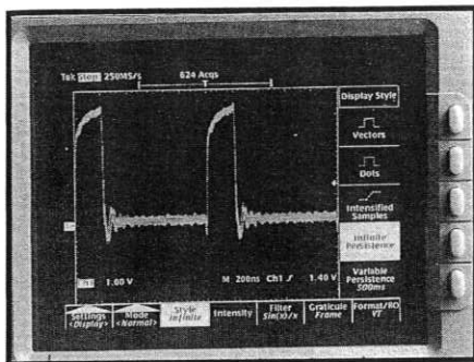
This waveform, captured in normal DSO mode, shows a well-behaved, repetitive digital waveform.
