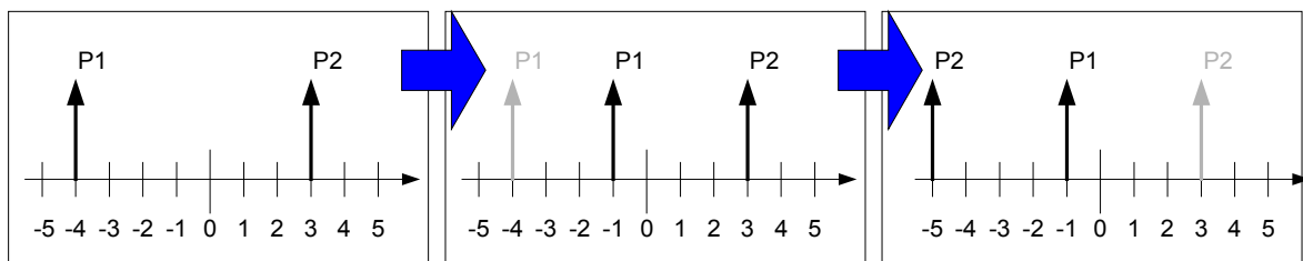
Fig. 2-44 Example of hop sequence with BIRTH-DEATH fading
