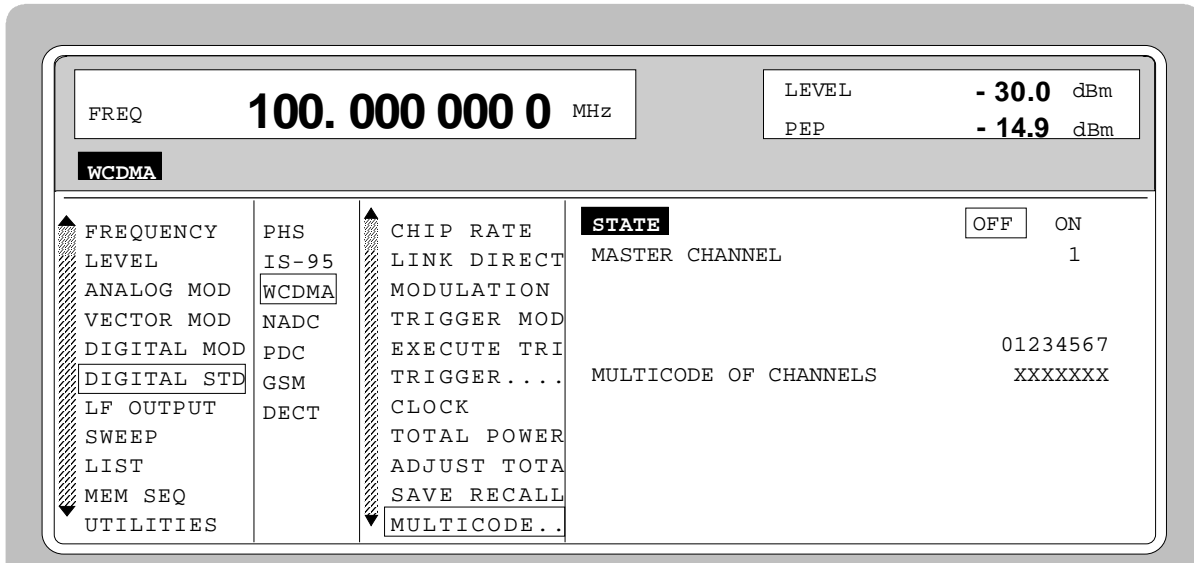
Fig. 2-93 Menu DIGITAL STD - WCDMA - MULTICODE..., equipped with options modulation coder SMIQB20, data generator SMIQB11 and SMIQB43
