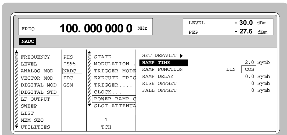
Fig. 2-180 Menu DIGITAL STD - NADC - POWER RAMP CONTROL... , SMIQ equipped with Modulation Coder SMIQB20 and Data Generator SMIQB11
