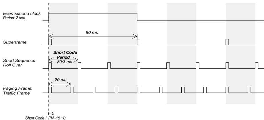
Fig. 2-80 CDMA sync signals
