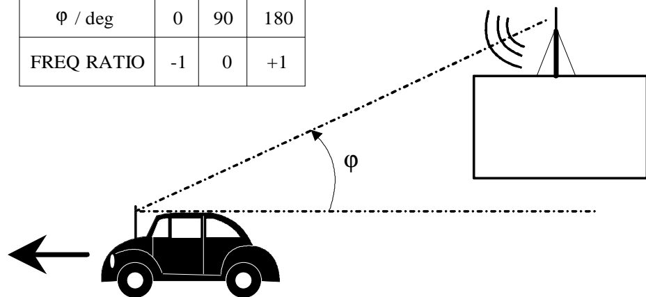
Fig. 2-40 Doppler Frequency shift with moving receiver
