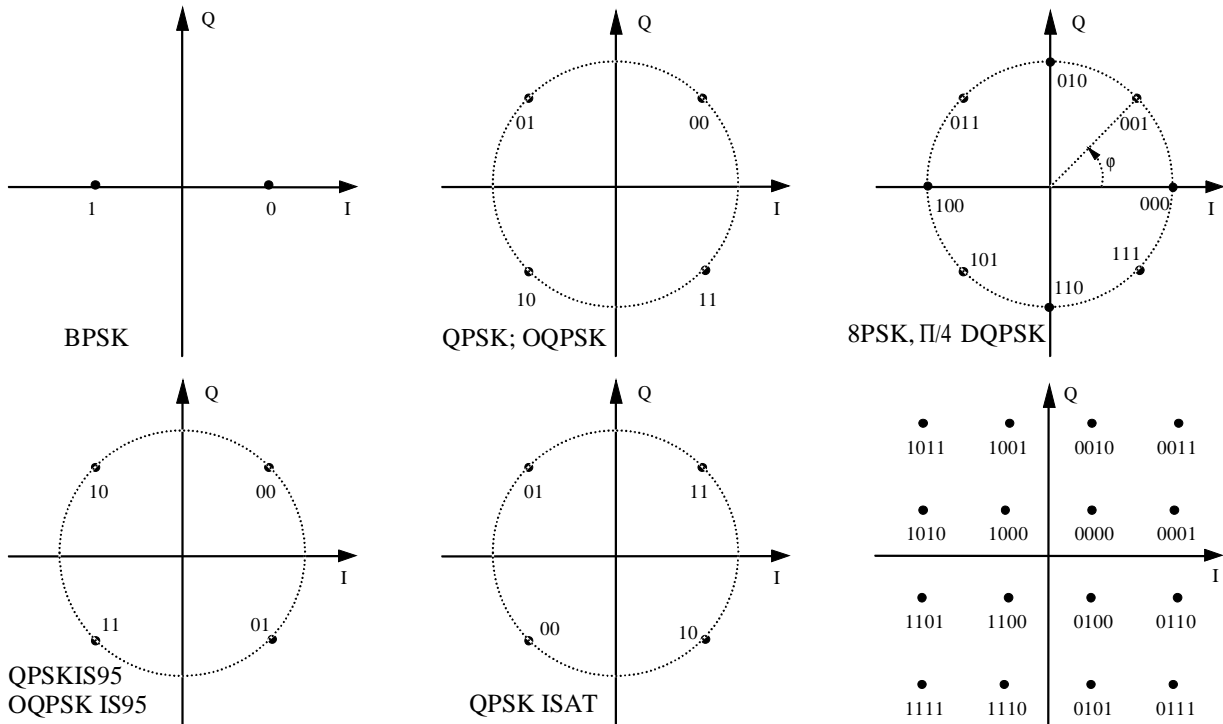
Fig. 2-50 Constellation diagrams of BPSK, QPSK, 8PSK and 16QAM
