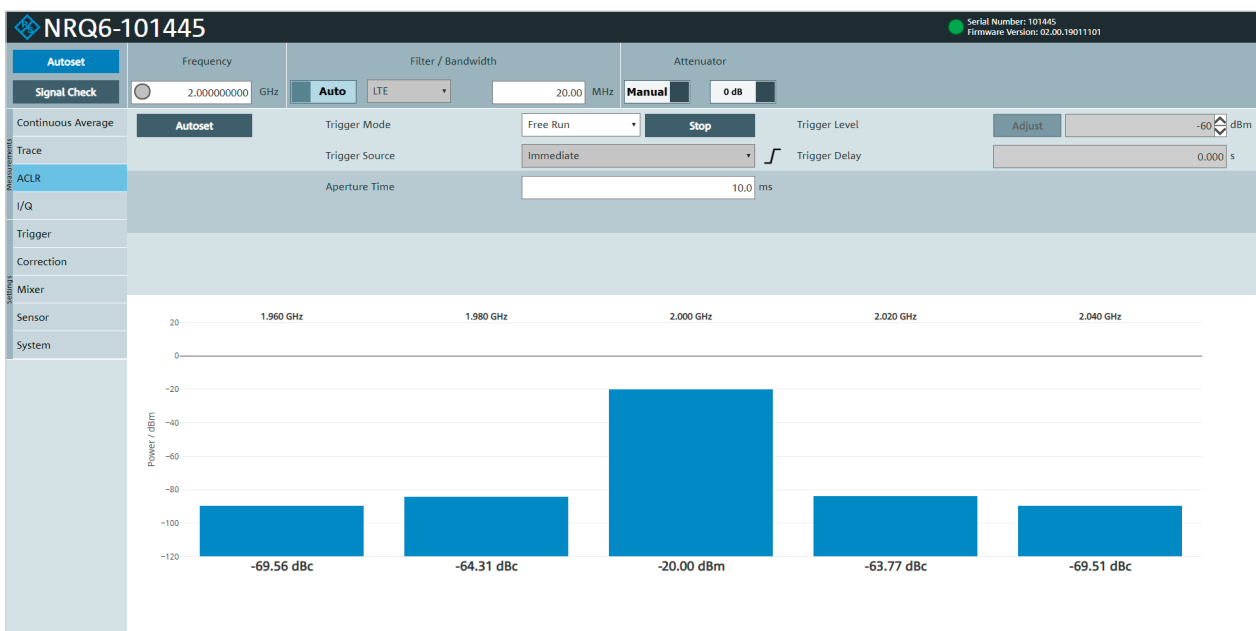
ACLR measurement on a 3.84 MHz 3GPP signal
