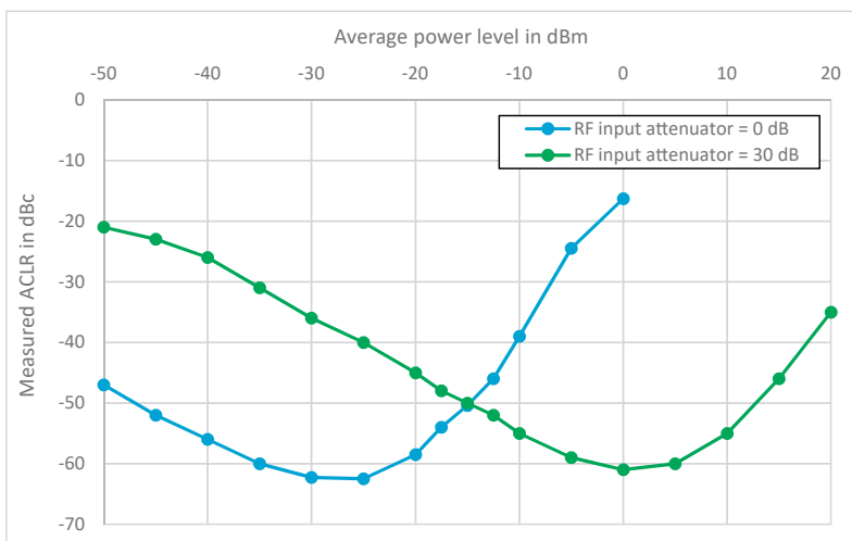
R&S®NRQ6 ACLR performance at 2 GHz over power; EUTRA/LTE 20 MHz (meas., noise correction on)
