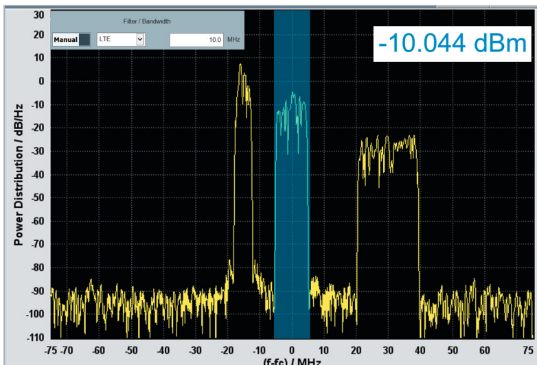
Single-channel power measurement on an MSR signal
