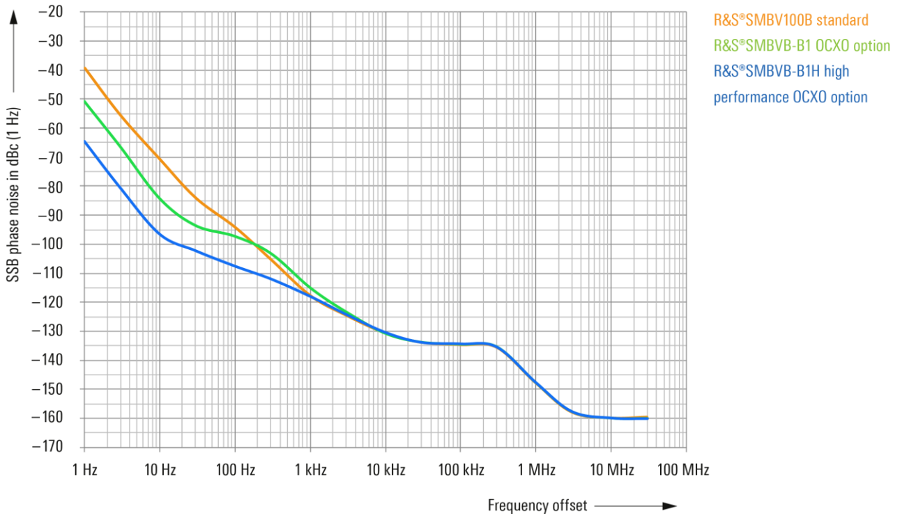
SSB phase noise comparison ( f = 1 GHz) with standard internal reference, R&S SMBVB-B1, R&S SMBVB-B1H (meas.).
