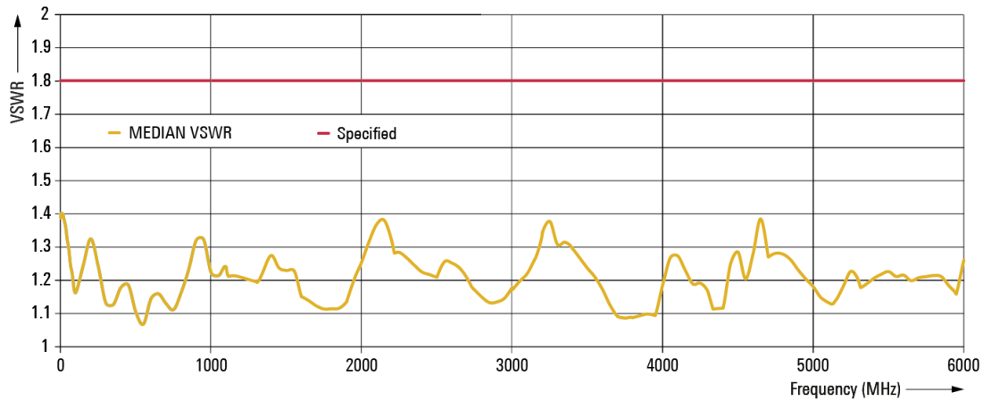
VSWR vs. frequency (with R&S®SMBVB-B32 option)
