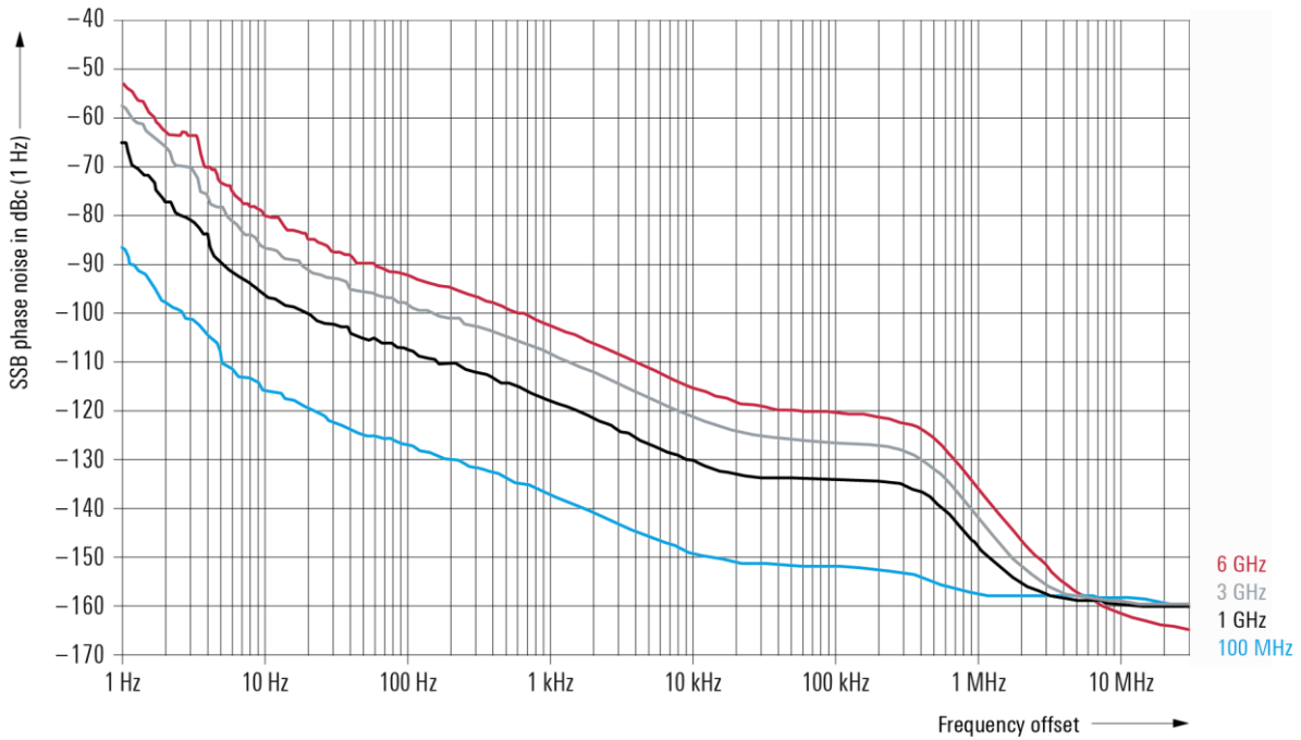
Measured SSB phase noise with R&S SMBVB-B1H option.
