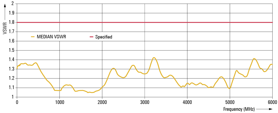
VSWR vs. frequency (without R&S®SMBVB-B32 option)
