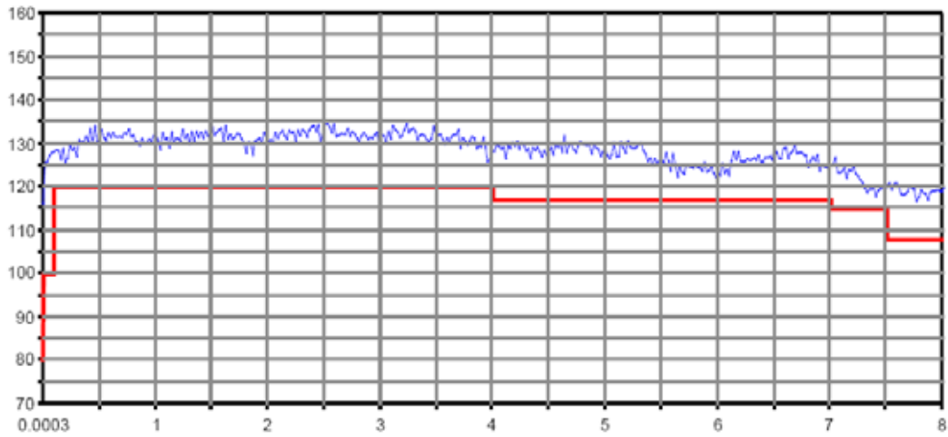
Dynamic range in dB versus frequency in GHz range of the R&S ZVB8
