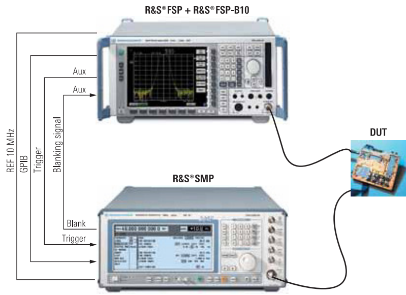
FIG 8: Scalar network analysis with the Microwave Signal Generator R&S®SMP and the Spectrum Analyzer R&S®FSP with option R&S®FSP-B10
