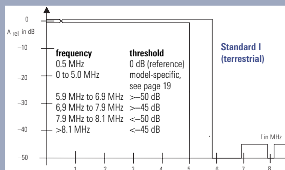
Tolerance masks of the R&S® EFA for total amplitude characteristic (RF, IF, VF)
