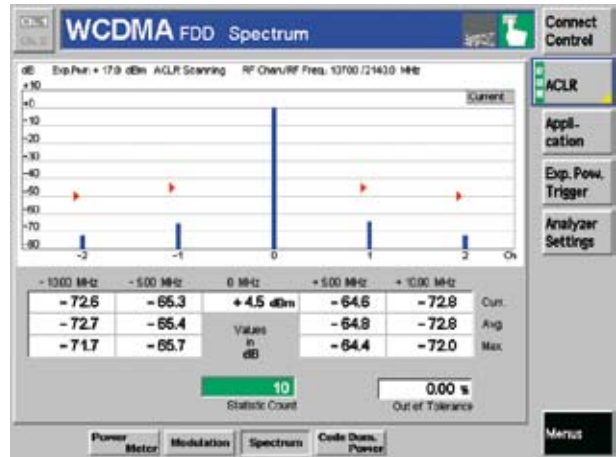
Adjacent Channel Leakage Ratio (ACLR) measurement.
