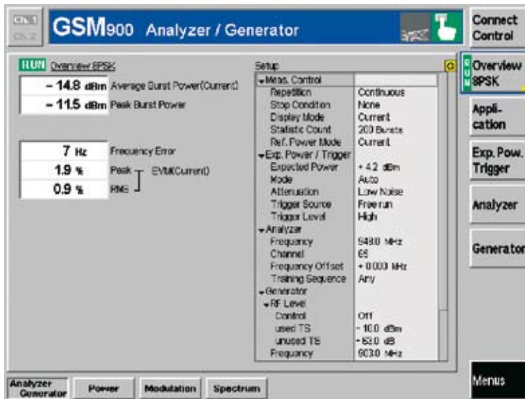
The non-signaling mode allows GMSK/8PSK signals to be generated and analyzed for RX/TX module testing; the hotkeys at the bottom of the screen provide immediate access to specific measurements.
