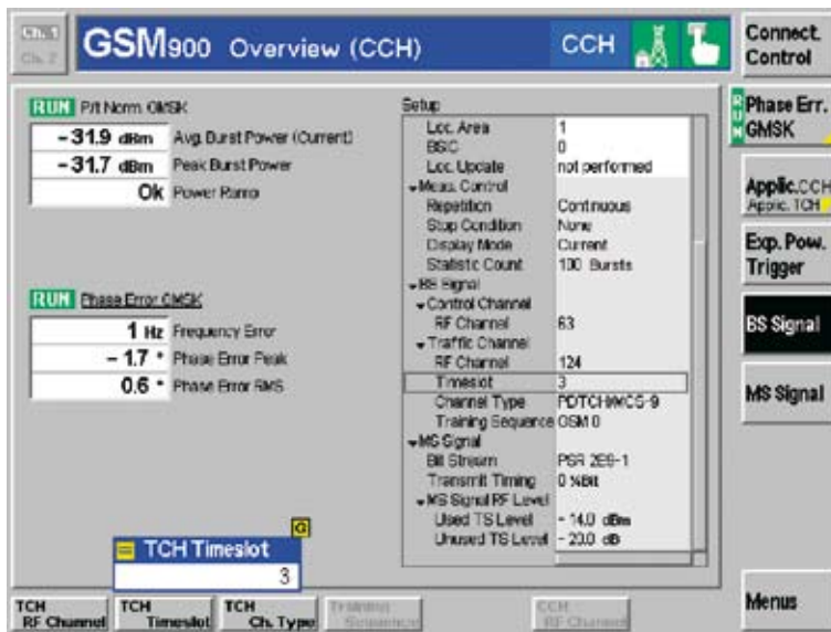
The signaling mode overview menu informs the user quickly and comprehensively about the BTS's TCH RF performance; timeslot-selective measurements are possible.
