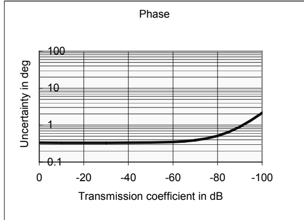
Typical accuracy of transmission magnitude and transmission phase measurements of the R&S®ZVB8 in the frequency range from 4 GHz to 8 GHz
