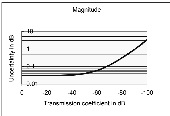
Typical accuracy of transmission magnitude and transmission phase measurements of the R&S®ZVB4 and the R&S®ZVB8 in the frequency range from 300 kHz to 4 GHz
