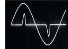
Same conditions as above with programmable Z_o engaged. THD=0.25%
