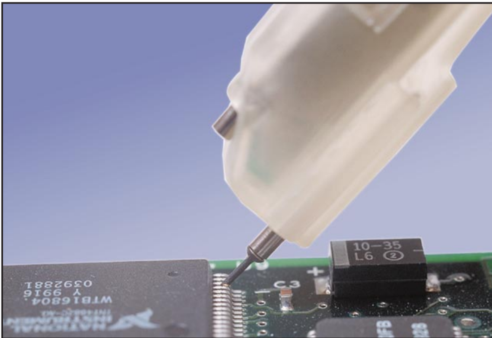
HFP Probe with IC Lead Tip on circuit board
