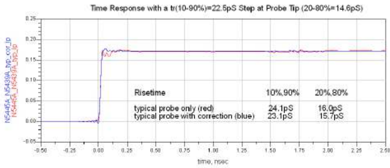
Time domain response plot with 1 mm span
