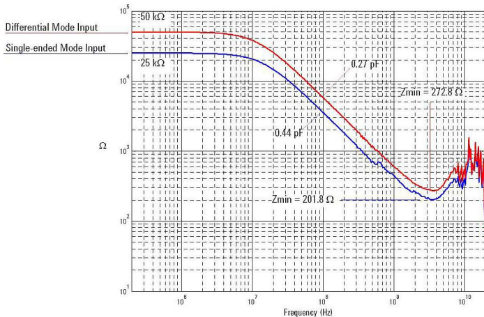
Probe input impedance vs. frequency
