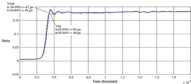
Graph of Vin and Vout of 1169A and N5381A solder-in head with a 25 Ω 58 psec step generator
