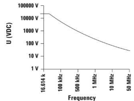
N2771B derating curve
