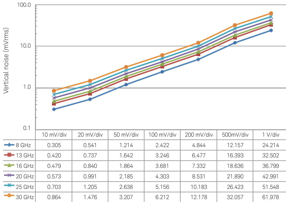
Noise of N7010A with Infiniium V-Series oscilloscopes
