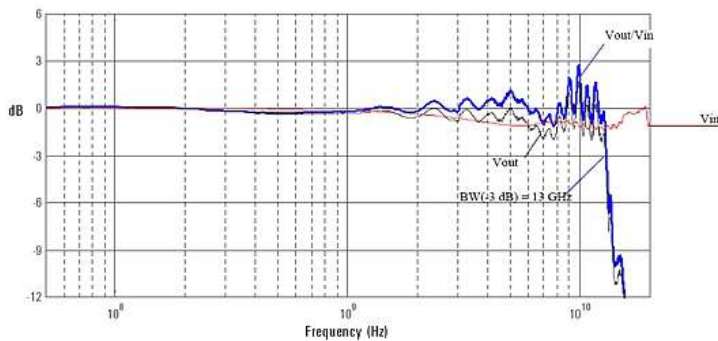
Frequency response of 1169A and N5381A with a 25 Ω source
