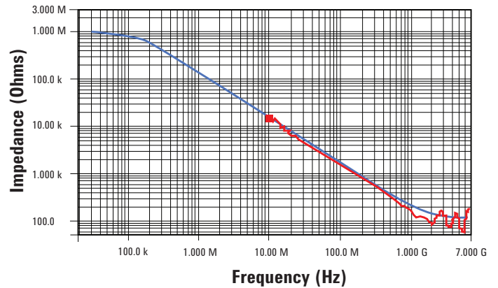
Input impedance over frequency (Red = measured, Blue = model)
