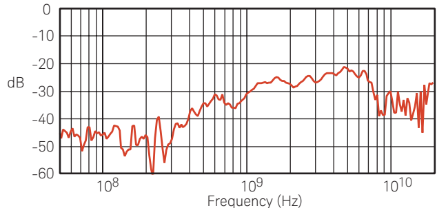
Common mode rejection versus frequency
