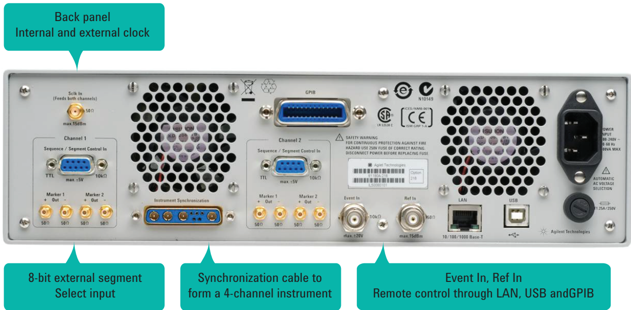
Figure 3. Back panel
