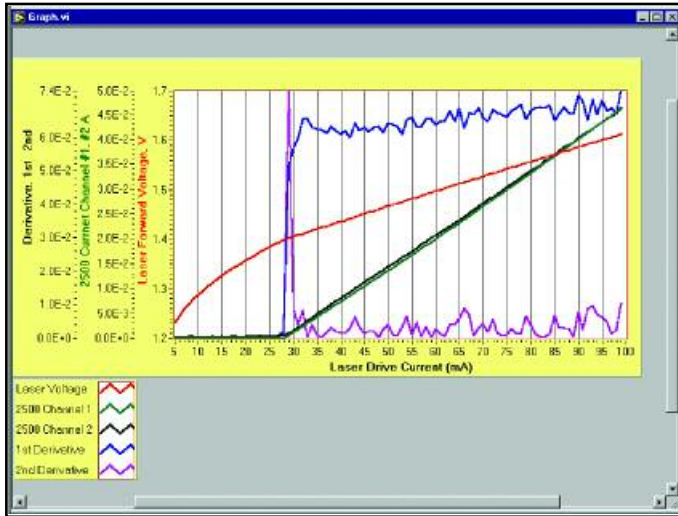
Figure 3. This plot illustrates the Model 2520's pulsed LIV sweep capability. The sweep was programmed from 0 to 100mA in 1mA steps. Pulse width was programmed at 1 \mu s at 1% duty cycle, providing for a complete sweep in just 10ms (excluding data transfer time).
