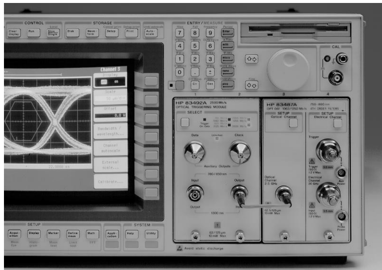
HP 83480A with the new HP 83492A Clock Recovery Module and HP 83487A Datacom Reference Receiver
