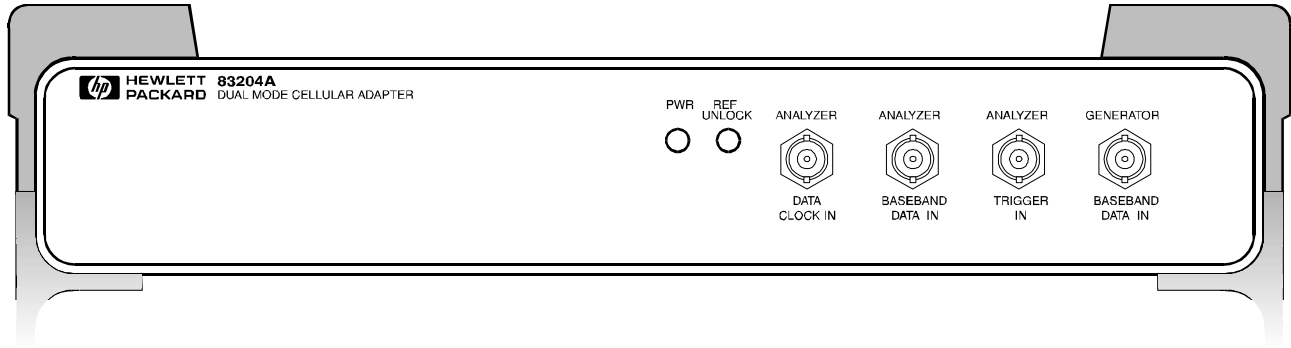
Front Panel
