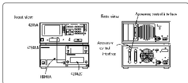
Bias current system configuration for 42842C
