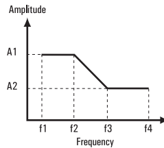
Bellcore GR-499 jitter amplitude versus modulation frequency:
