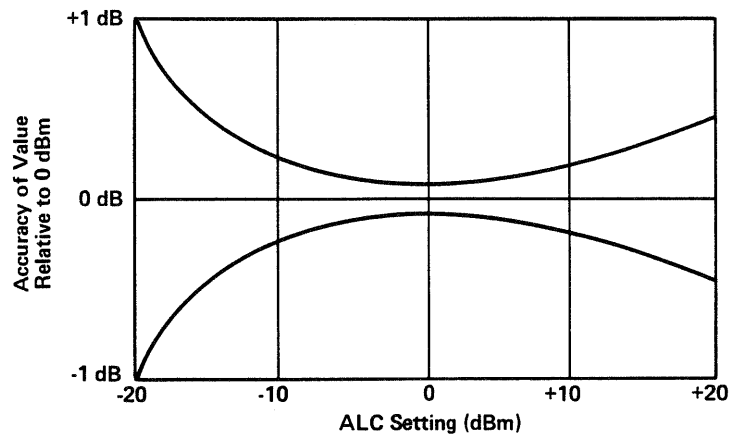
Figure 2. Typical ALC Incremental Accuracy
