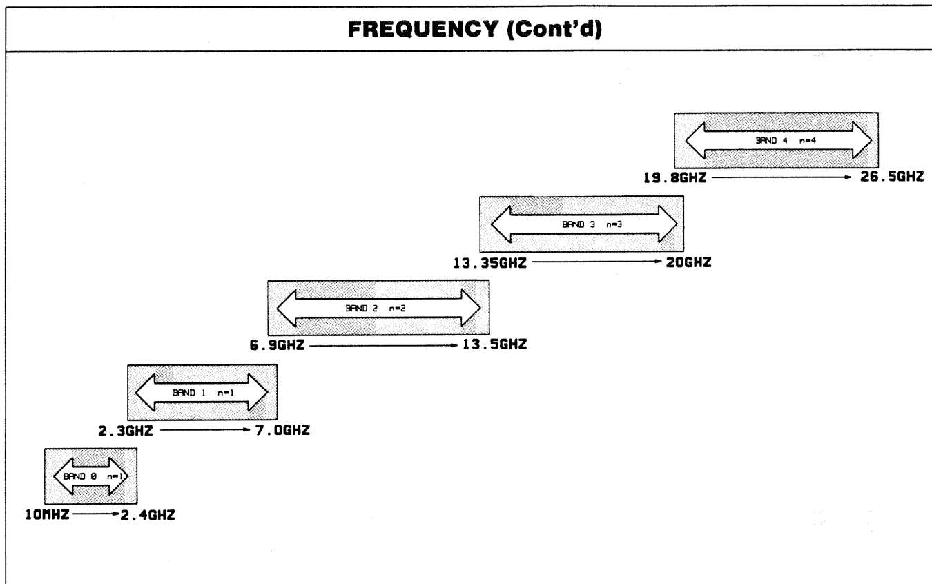
Figure 1. Typical Frequency Ranges and Bandswitch Points in Swept Modes
