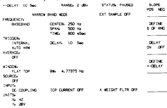
Figure 7: Plots of the view state display provide quick hard copy of instrument setup for complete measurement documentation.
