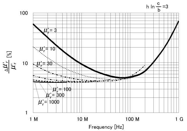
Figure 23. Permeability accuracy \frac{(\Delta\mu')}{\mu'} vs. frequency (at F = 3 , typical)
