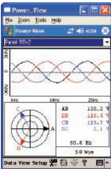
View measurements real-time with wireless PDA interface.
