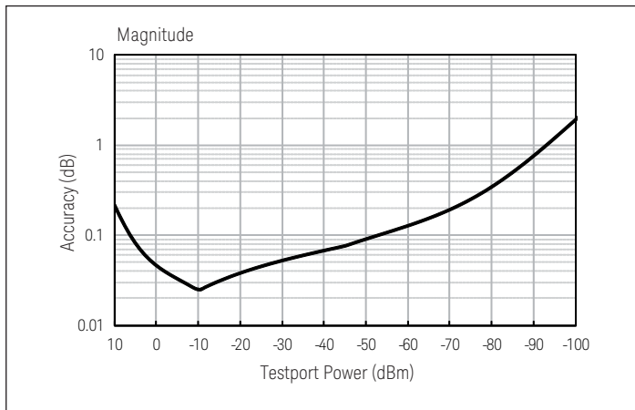
Figure 10. Dynamic Accuracy
