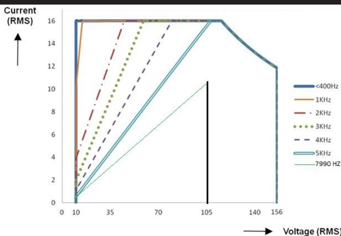
Current Frequency Rating Chart for 156VAC Range (range in 3 phase mode)
