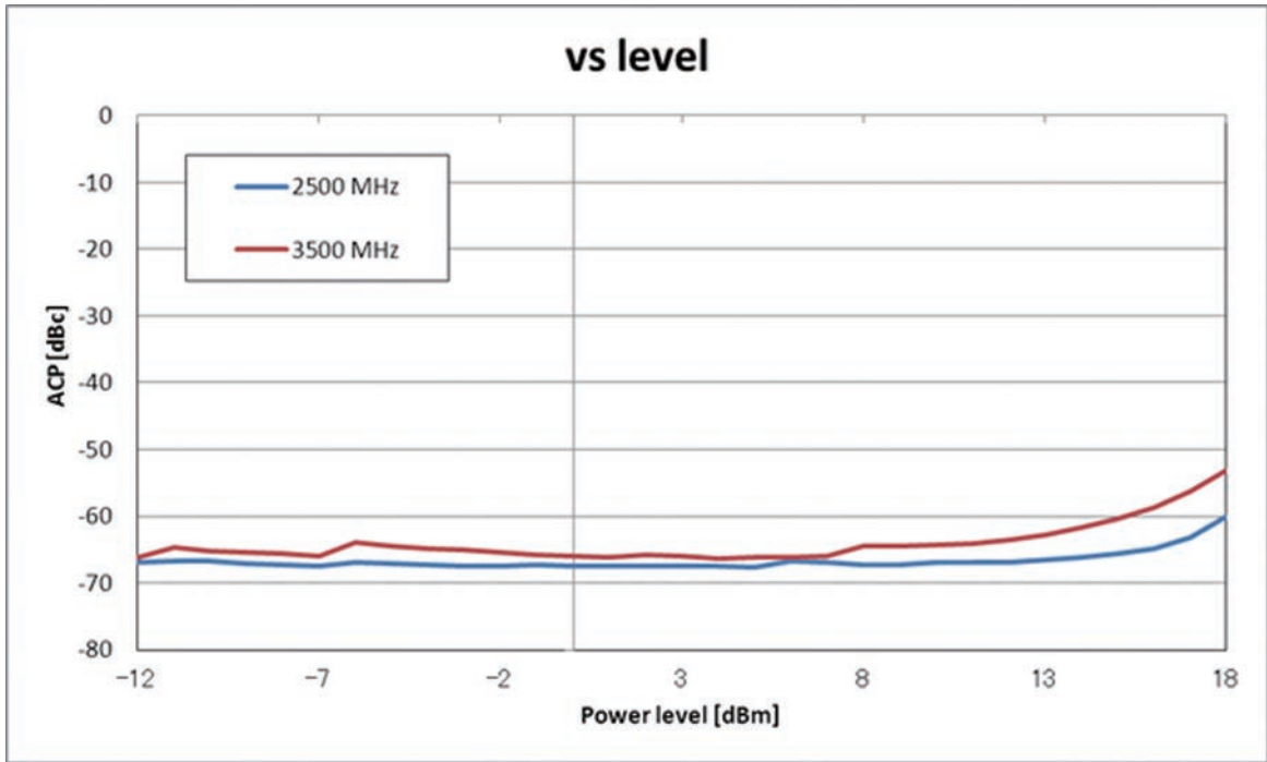
ACP vs. Power level (10 MHz offset, with MG3710A-041)
