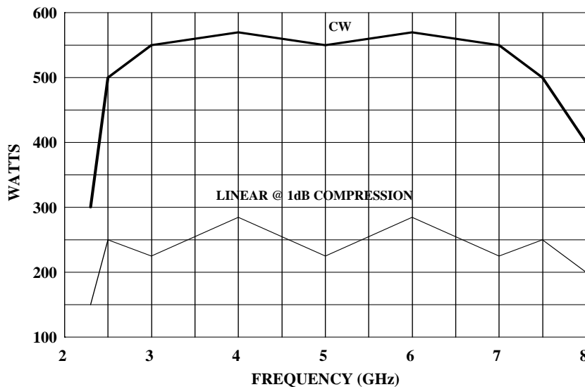
500T2z5G7z5 TYPICAL POWER OUTPUT
