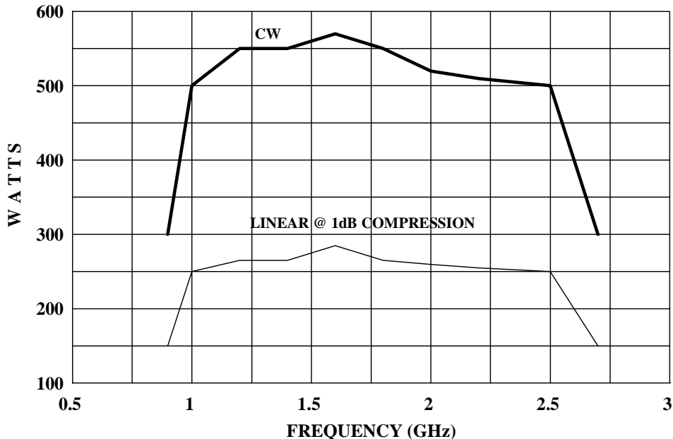
500T1G2 TYPICAL POWER OUTPUT
