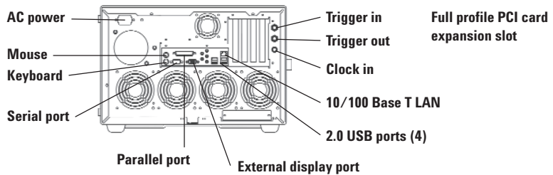
Figure 9. 16800 Series back panel
