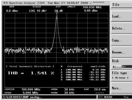
Harmonic Distortion
