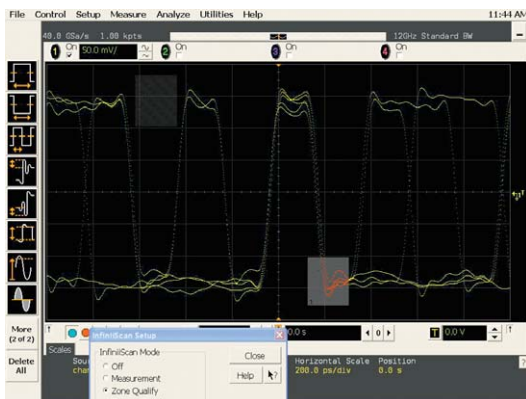
The "true" ease of use. Just draw boxes and the scope will trigger. The industry's only software event finder, "InfiniScan Event Identification Tool" will provide the next level of ease-of-use for the scope triggering system.
