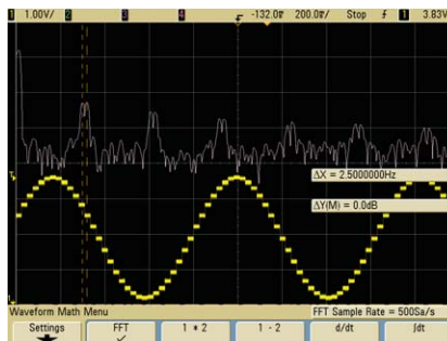
Figure 10. FFT allows you to view the spectral content of this unfiltered sine wave
