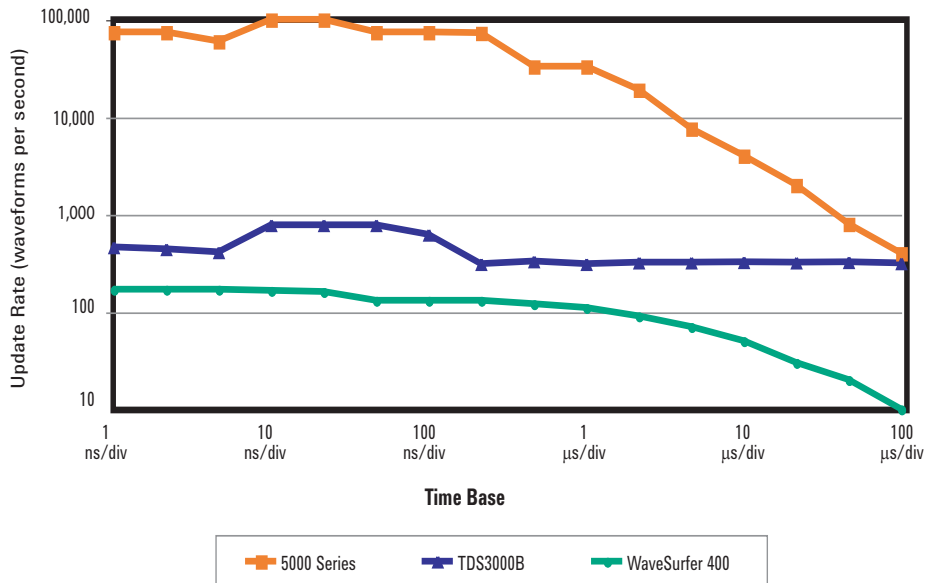
Figure 5. Update rates of popular oscilloscopes using their default real-time time acquisition mode
