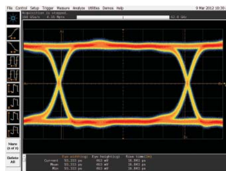
10 Gbps signal captured with 62 GHz of bandwidth, notice the faster rise time and wider eye measurements
