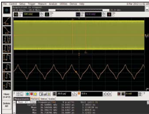
Use EZJIT software to extract spread spectrum clocks
