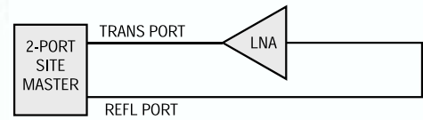
Amplifier Gain Test Measurement.
