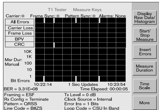
T1/E1 Measurement using Option 50
