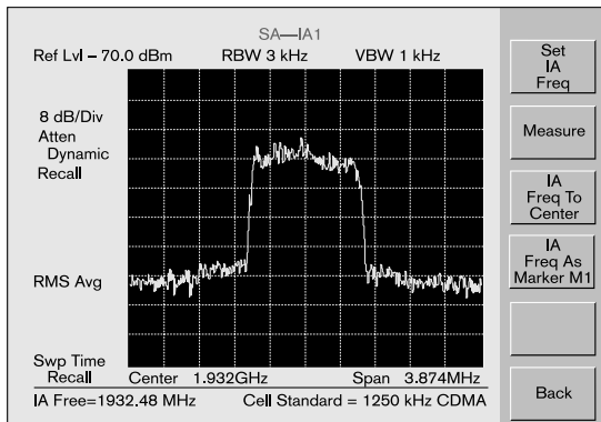
Interference Analysis S332D
