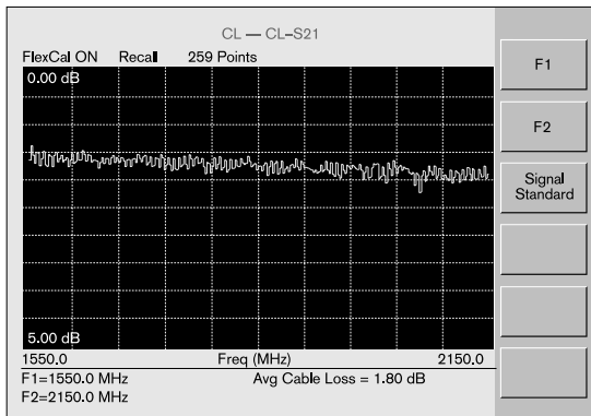
Cable Loss
