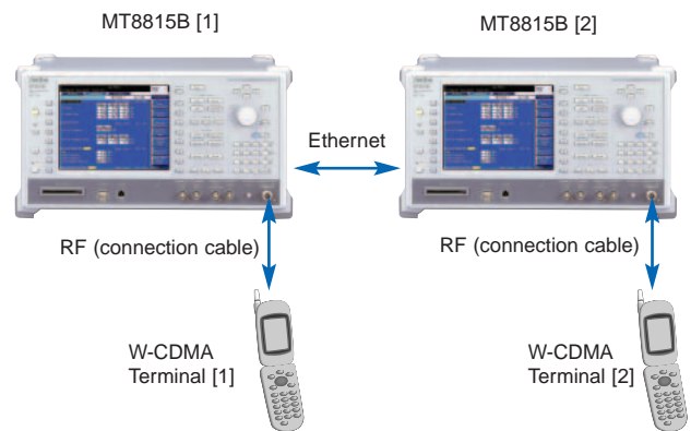
Sample MT8815B connection: when MT8815B is two sets
