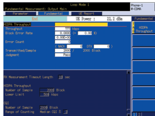
Throughput
