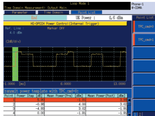
HS-DPCCH Measurement
