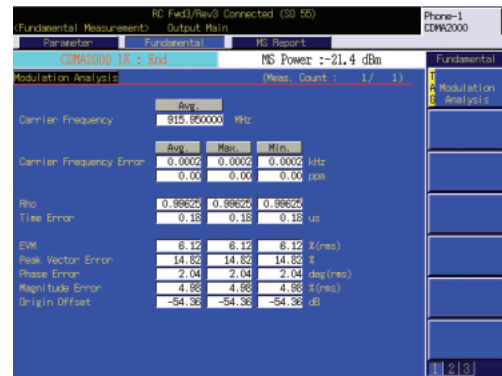
Modulation Analysis
