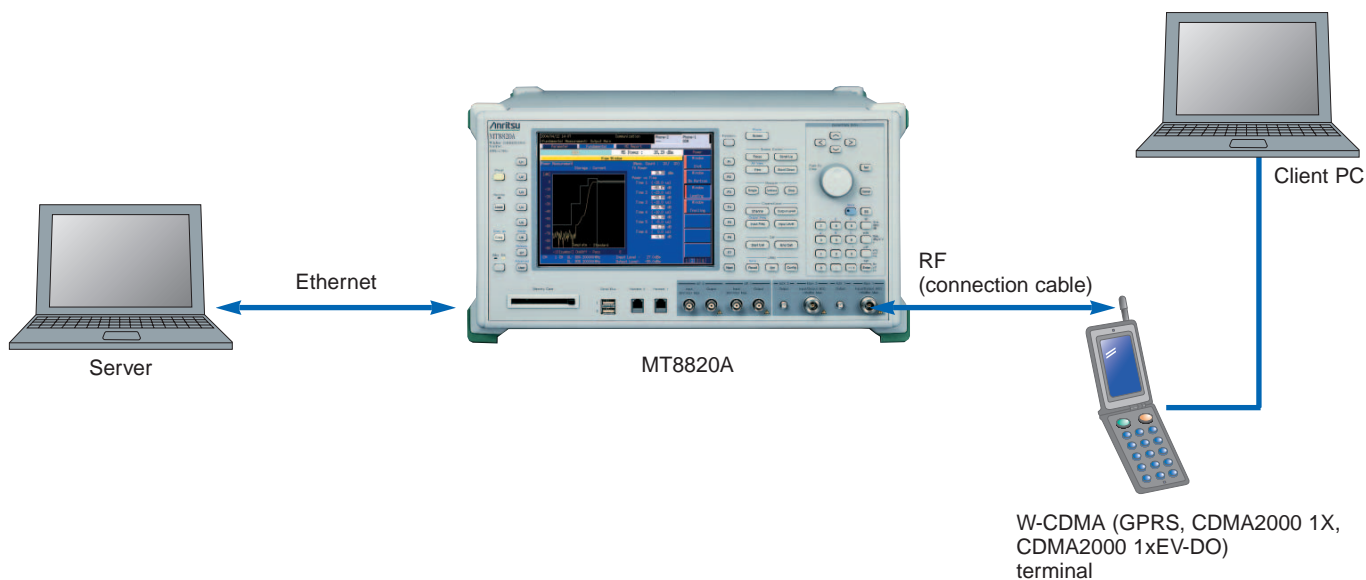
Sample MT8820A connection
